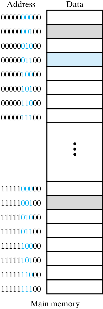
(b) Cache mapping
